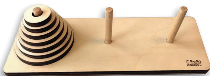
HANOI TORANJ
